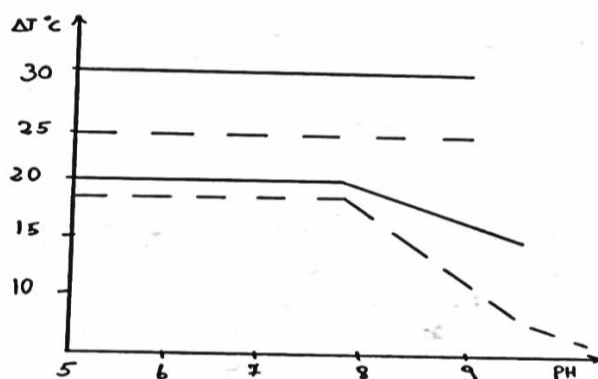
Fig.1. The effect of tanning solution pH and washing in an acidic environment on the change in dermis boiling temperature
