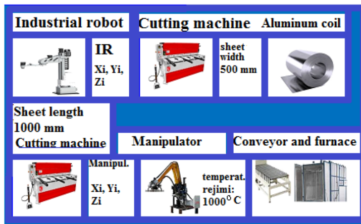
Fig. The block diagram of the real technical control system of each production module of the FMS is displayed on the screen of the operator's monitor
